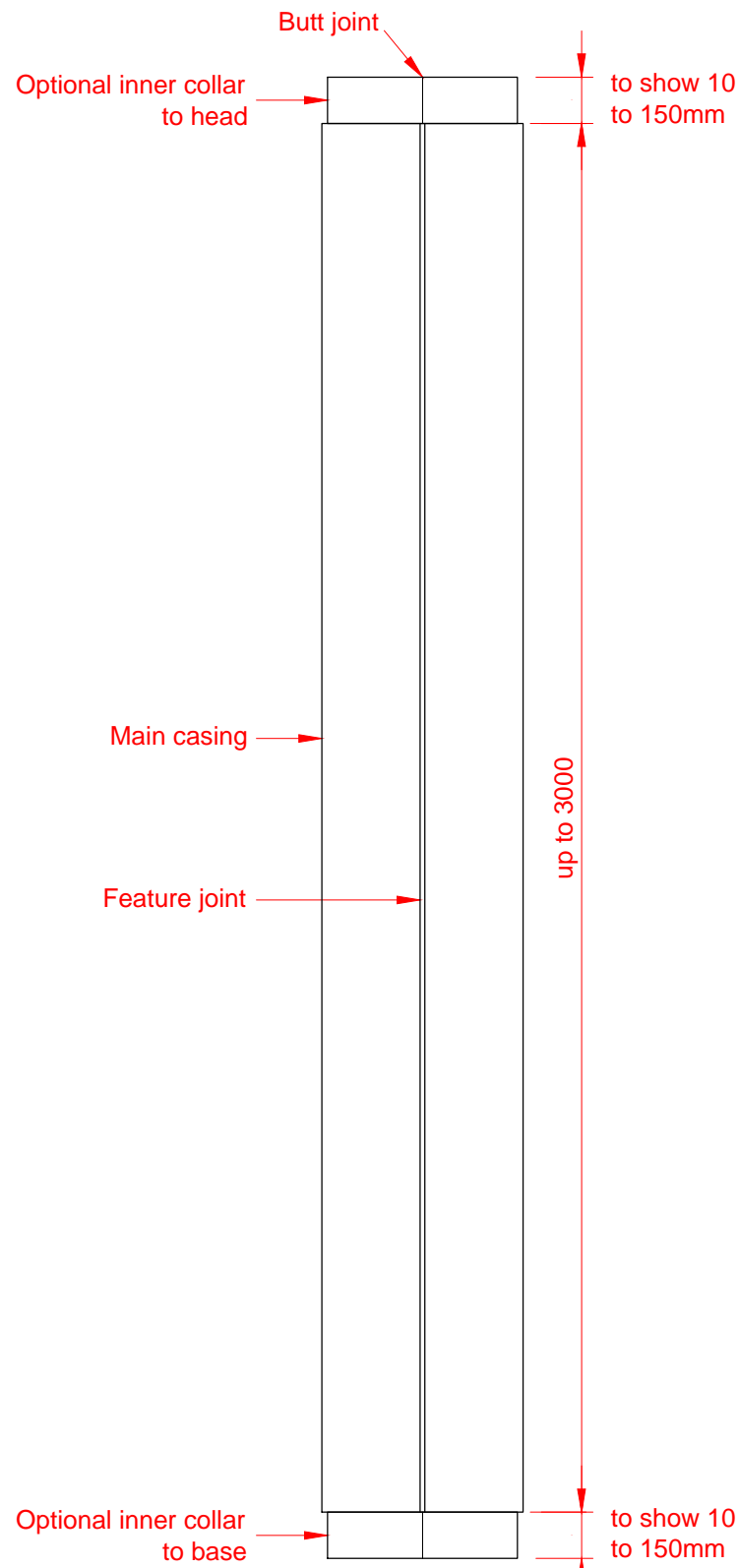
STANDARD ELEVATION UP TO 3300 HIGH
