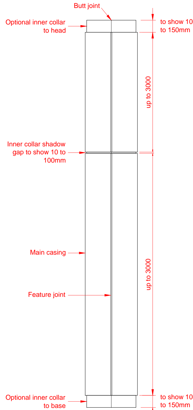
STANDARD ELEVATION BETWEEN 3300 & 6400 HIGH
