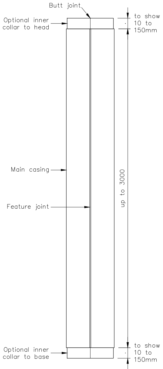
STANDARD ELEVATION UP TO 3300 HIGH
