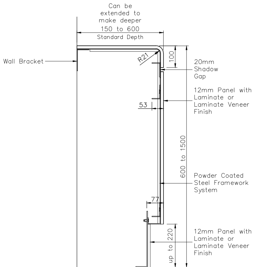
PCMX Type A Available in upto 3m lengths in one section
